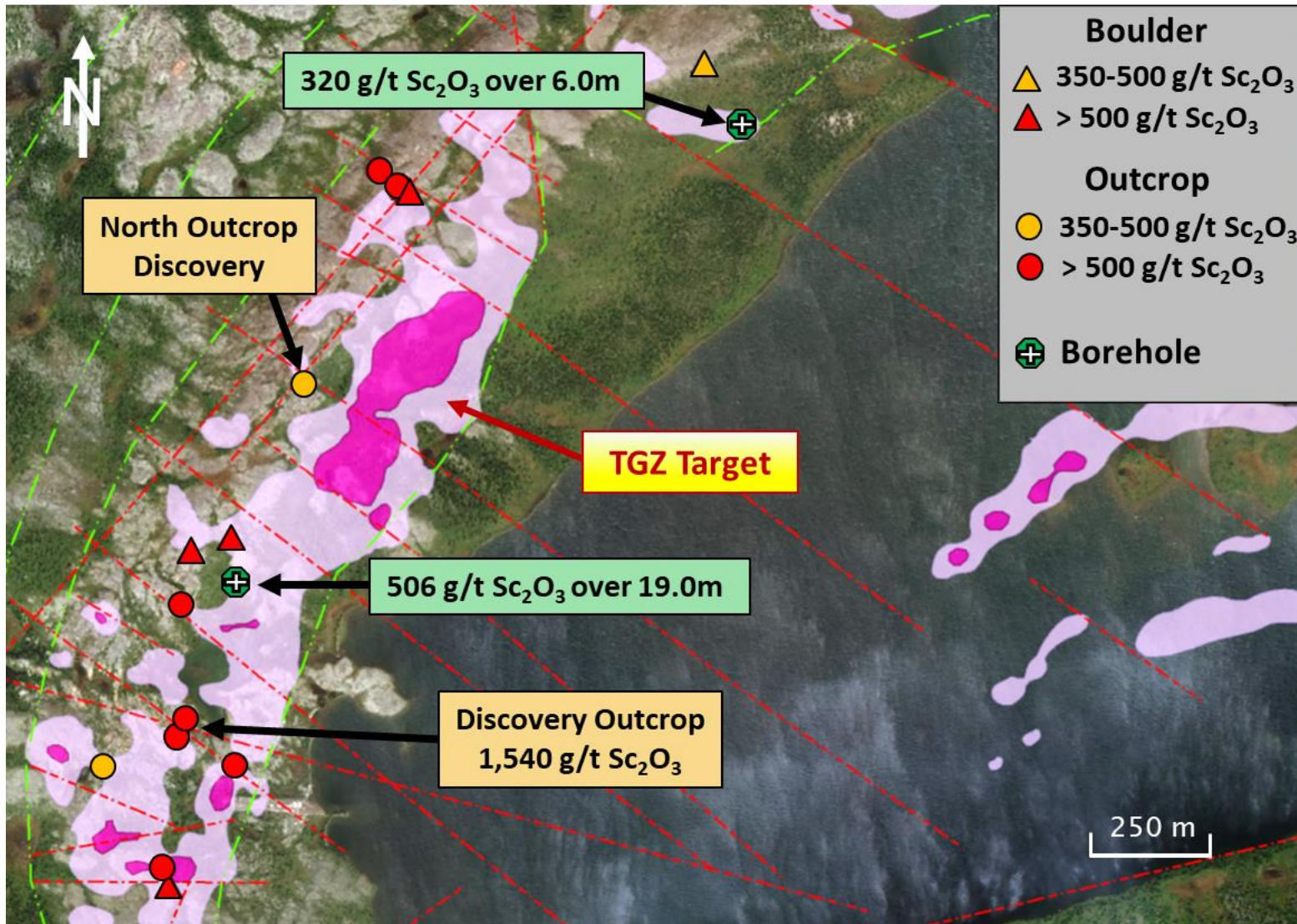
Figure 3 – TG Zone Proposed Diamond Drilling, Crater Lake Project, Quebec
