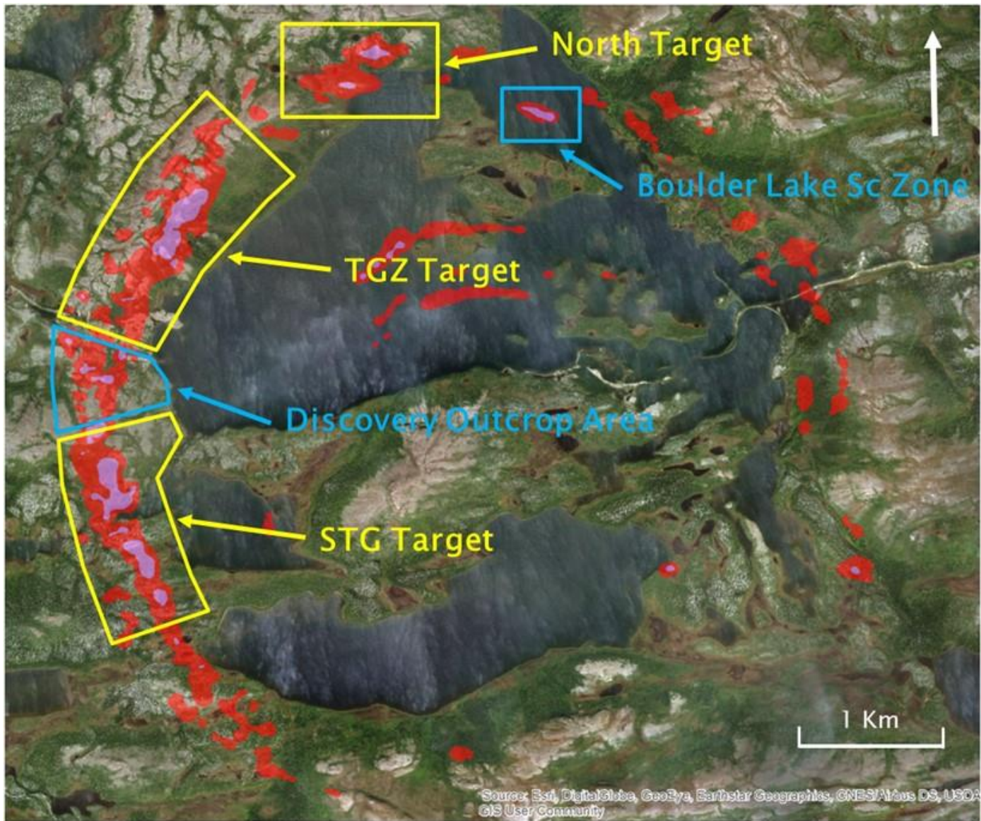
Figure 2 – Exploration Targets over Ground Magnetic Map, Crater Lake Project, Québec
