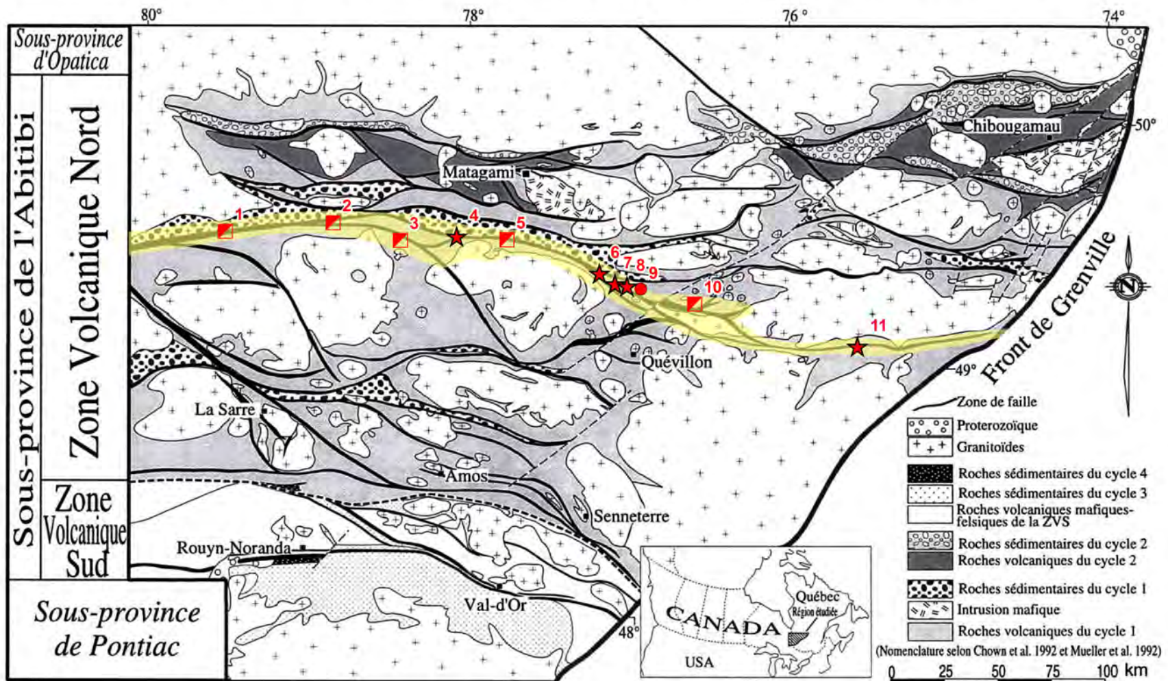
Figure 3 - Geologic map of the Abitibi sub-province (after Chown et al 1992)
