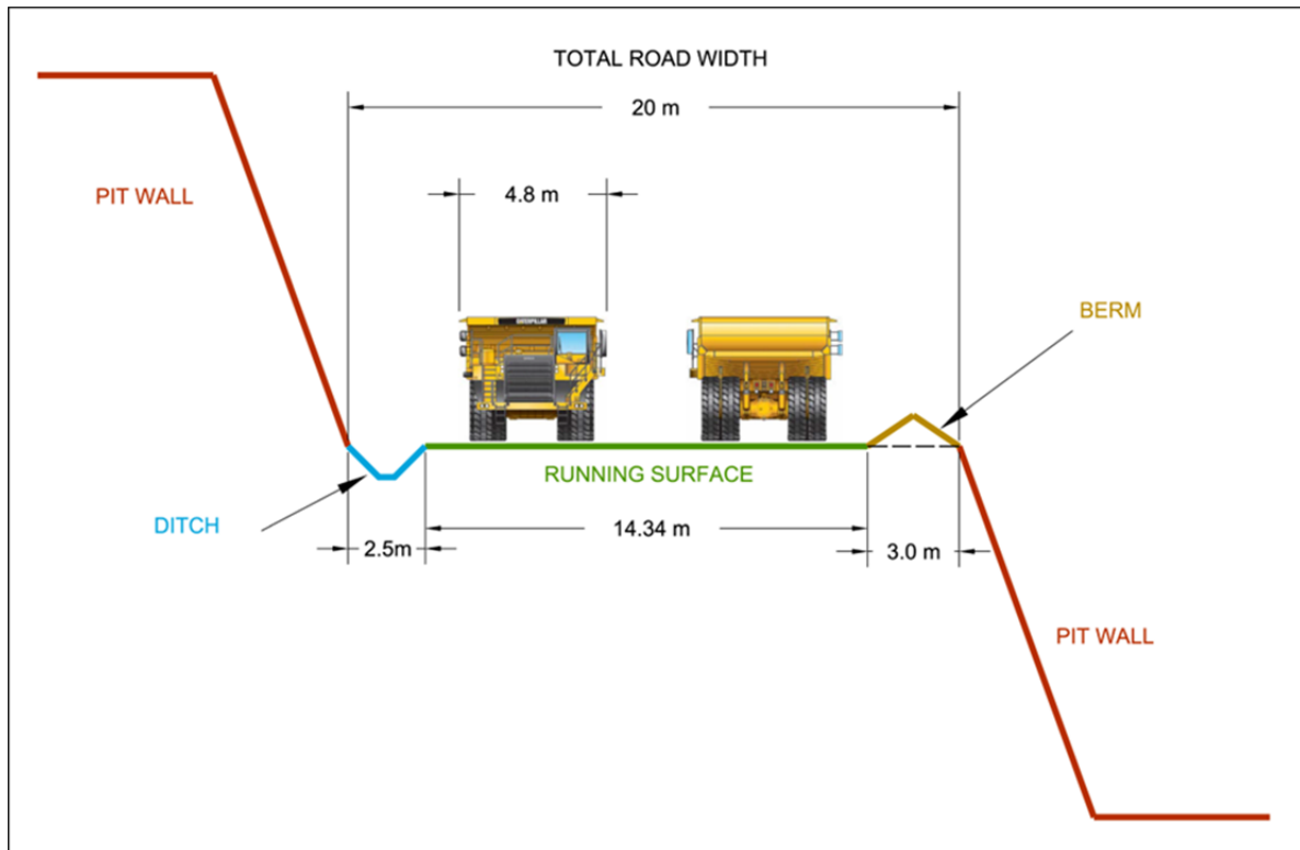
Figure 16-8: Ramp Design
